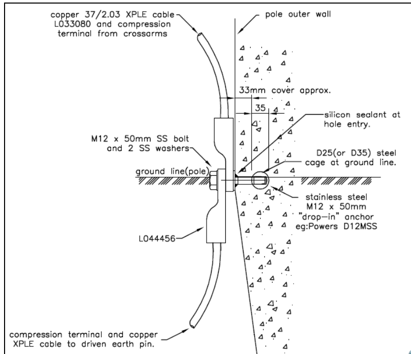
Figure 3: Bonding details for Vierendeel poles.
