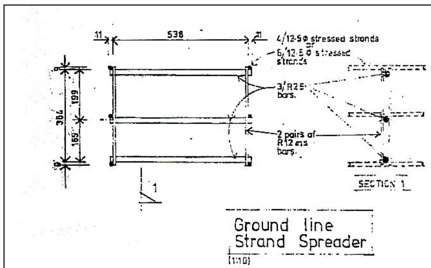
Figure 2: Vierendeel pole ground line spreader cage
