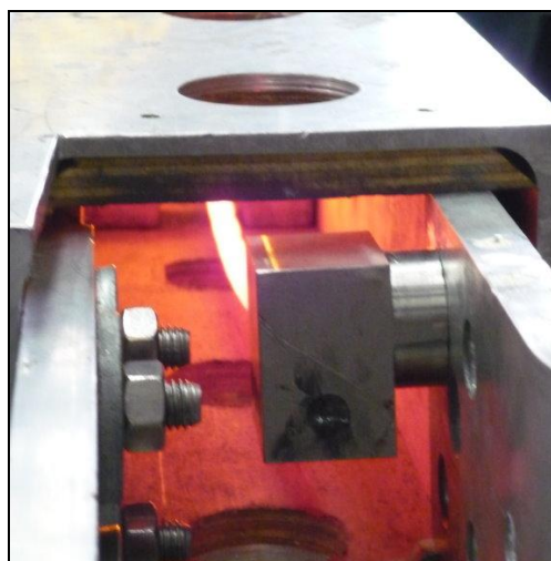
Figure 11: Strand white hot where it emerges from connection ferrule
